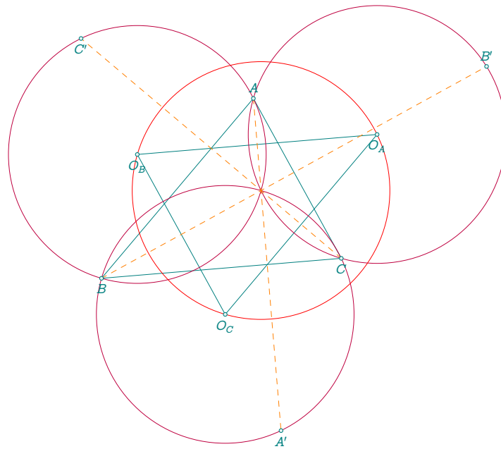
33.63 Yiu's circles variant two
