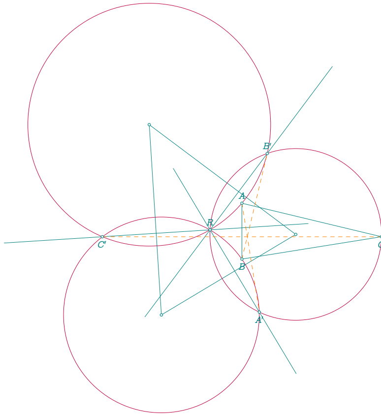
33.63 Yiu's circles variant two
